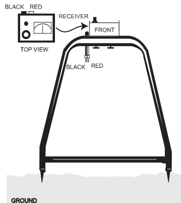
Figure 2. Receiver Setup
