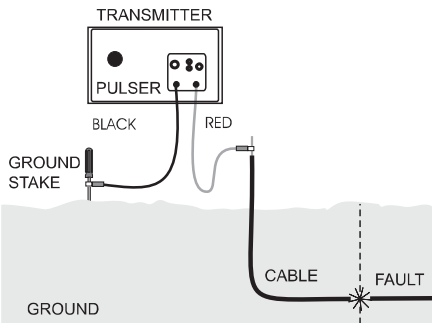
Figure 1. Transmitter Setup
